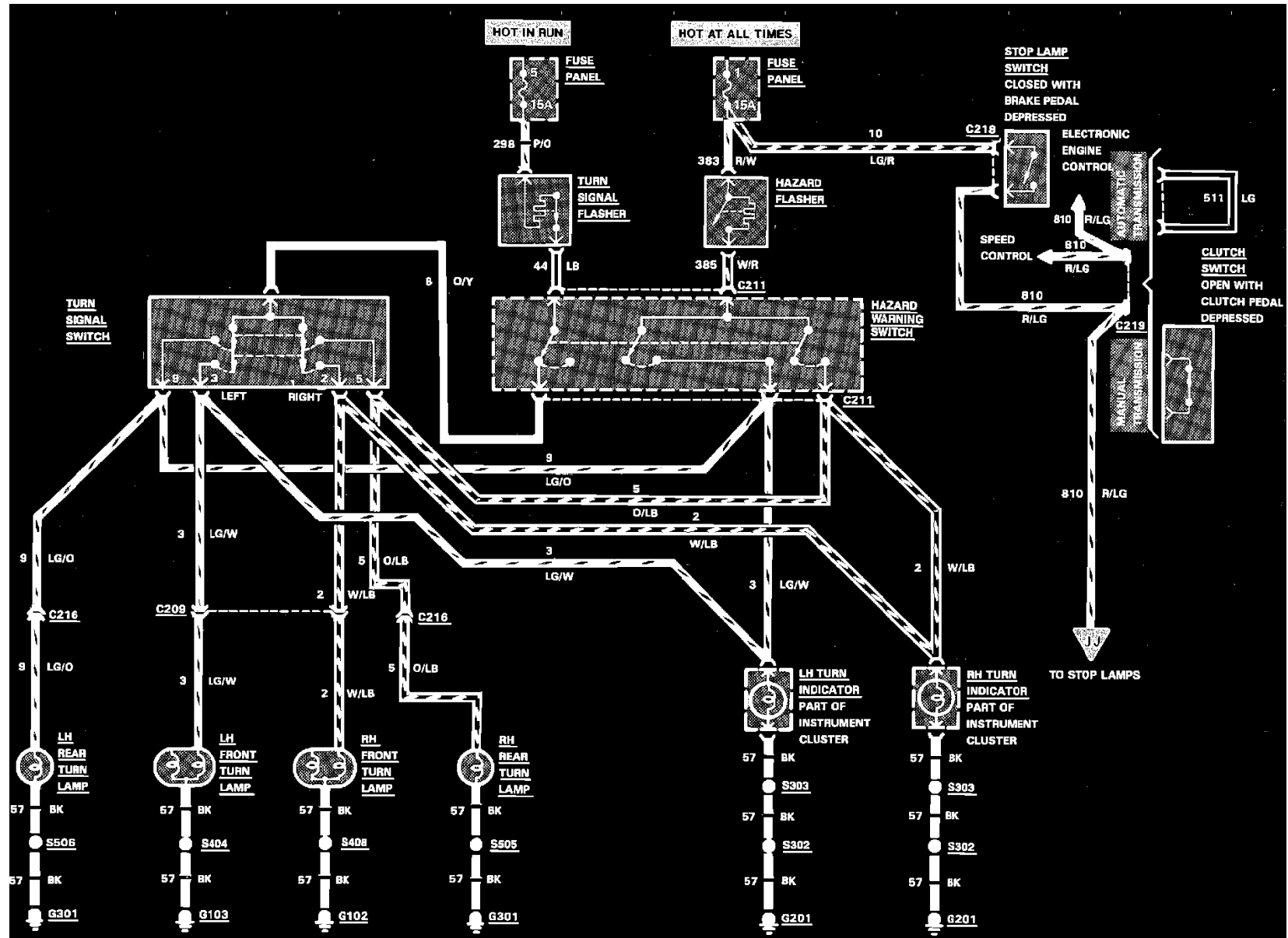
Hazard, Stop & Turn Lamp Wiring Circuit
