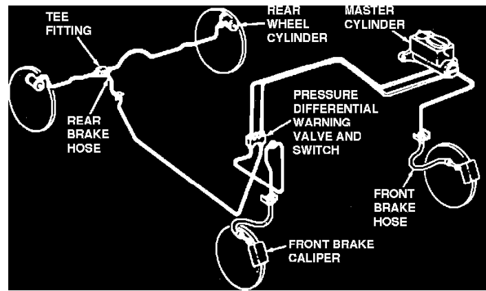
Fig. 1 Schematic Diagram Of A Typical Hydraulic Front & Rear Split Brake System
