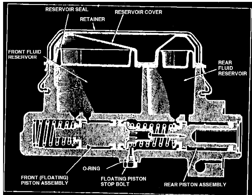
Fig. 2 Bendix dual master cylinder (Typical)
