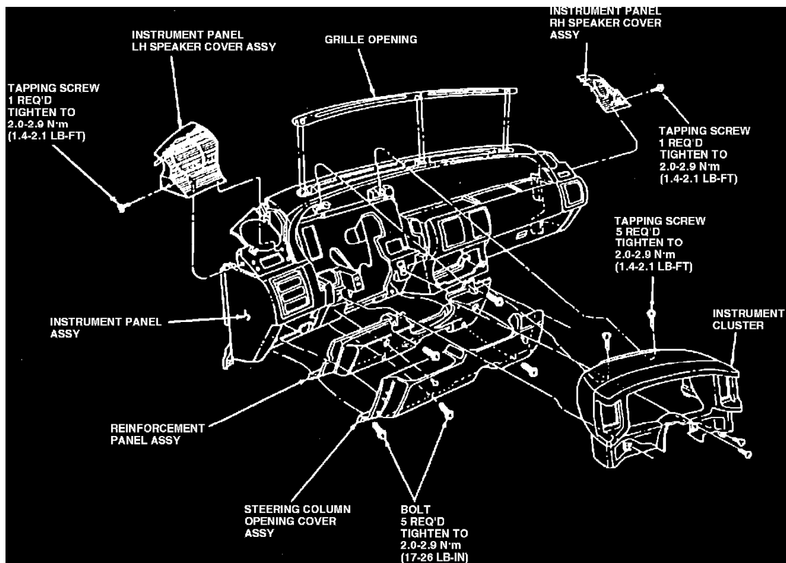
Fig. 51 Exploded View Of I/P. 1990-91 Mustang
